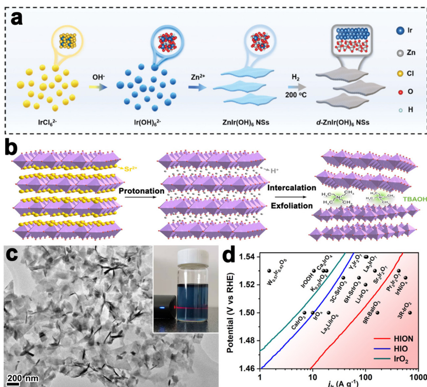
Fig. 5 (a) Schematic illustration of the synthesis of \text{ZnIr(OH)}_6 NSs and d\text{-ZnIr(OH)}_6 NSs (reproduced from ref. 92 with permission from the Royal Society of Chemistry, copyright 2022). 92 (b) Liquid-phase exfoliation of \text{Sr}_2\text{IrO}_4 . (c) TEM image of HION and the inset showing the photograph of HION colloidal suspension with typical Tyndall light scattering under laser irradiation. (d) Comparison of Ir mass activity of HION with previously reported OER catalysts in acid media (reproduced from ref. 93 with permission from the American Chemical Society, copyright 2022). 93
