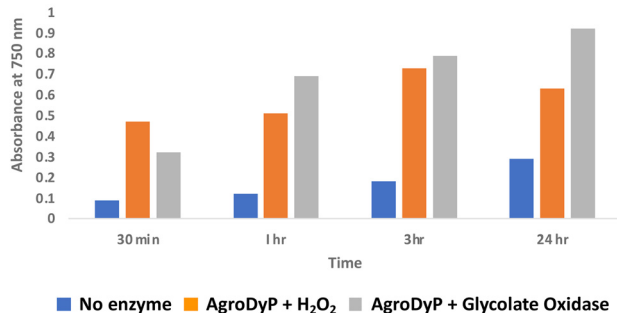
Fig. 5 Formation of low molecular weight ketone/aldehyde products via 2,4-dinitrophenylhydrazine assay (A) and phenolic products via Folin–Ciocalteu assay (B) from conversion of poplar alkaline organosolv lignin by Agrobacterium DyP/1 mM hydrogen peroxide (in orange) vs. Agrobacterium DyP/ R. jostii glycolate oxidase/1 mM glycolic acid (in grey). Assay data for conversion of other polymeric lignins are shown in ESI.†
