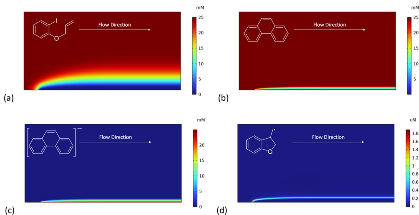
Fig. 9 Flow simulation for electroreduction of 1 in the presence of phenanthrene ( M , 1 equiv.). Concentration heat maps for: (a) Arl 1 . (b) Phenanthrene ( M ). (c) Phenanthrene radical anion ( M •- ). (d) Cyclised radical intermediate 6 . Starting concentration of Arl 1 is 0.025 M. Electrolysis time = 0 to 2.4 s under constant potential of -2.8 V vs. SCE.
