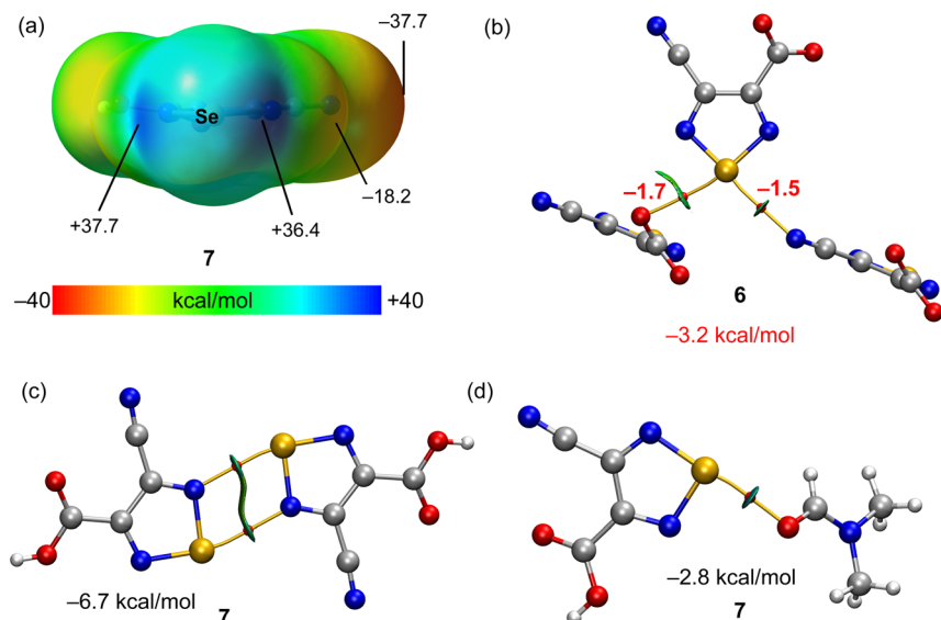
Fig. 5 (a) MEP surface of compound 7 with indication of the MEP maximum and minimum and other selected points of the surface. Energies in kcal mol -1 . (b–d) QTAIM (bond critical points in red and bond paths as orange lines) and NCIPlot (RDG = 0.4, density cut-off = 0.04 a.u., color scale \pm 0.04 a.u.) representation for compounds 6 and 7. Only intermolecular interactions are represented. The association energies in kcal mol -1 of the chalcogen bonds derived from V_r are given in red adjacent to the bond CP.
