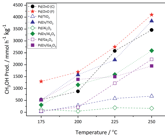
Fig. 1 Methanol productivity as a function of \text{CO}_2 hydrogenation reaction temperature over calcined Pd and PdZn supported catalysts. Pd/ZnO(C) is Pd supported on the commercial support, whereas Pd/ZnO(F) is Pd supported on the Farag-style ZnO.
