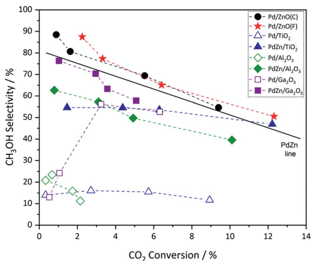
Fig. 2 Plot of \text{CO}_2 conversion vs. \text{CH}_3\text{OH} selectivity over calcined Pd and PdZn supported catalysts. The four data points for each entry correspond to the increasing reaction temperature (left to right) from 175 to 250 ^\circ\text{C} , corresponding with increasing conversion. The line shown is that reported recently for a range of PdZn catalysts. 24
