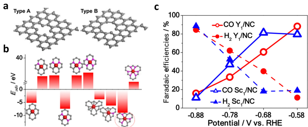
Fig. 8 (a) Structural diagram of type A and type B substrates with small-size and large-size carbon defects, respectively. (b) Calculated adsorption energies of different active sites of Y/NC. (c) FE_{CO} and FE_{H_2} of Y/NC and Sc/NC from -0.58 V to -0.88 V. Reproduced with permission. 67 Copyright (2020) American Chemical Society.
