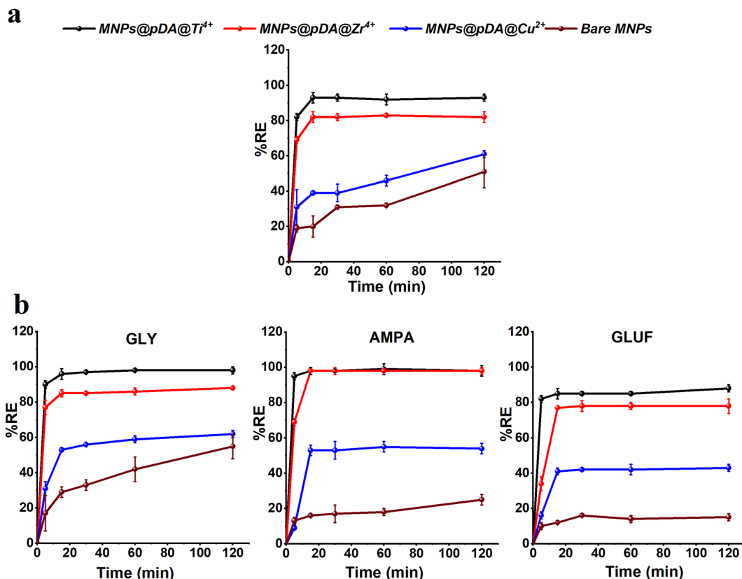
Fig. 6 Influence of incubation time on the RE% of the MNPs ( 100 \text{ mg L}^{-1} ) for a) GLY 500 \text{ } \mu\text{g}_{\text{GLY}} \text{ g}_{\text{MNPs}}^{-1} , and b) GLY 200 \text{ } \mu\text{g}_{\text{analyte}} \text{ g}_{\text{MNPs}}^{-1} (in a mixture), AMPA 200 \text{ } \mu\text{g}_{\text{analyte}} \text{ g}_{\text{MNPs}}^{-1} (in a mixture), and GLUF 200 \text{ } \mu\text{g}_{\text{analyte}} \text{ g}_{\text{MNPs}}^{-1} (in a mixture), at room temperature. Data are reported as mean \pm S.E.M. ( n = 3 ).
