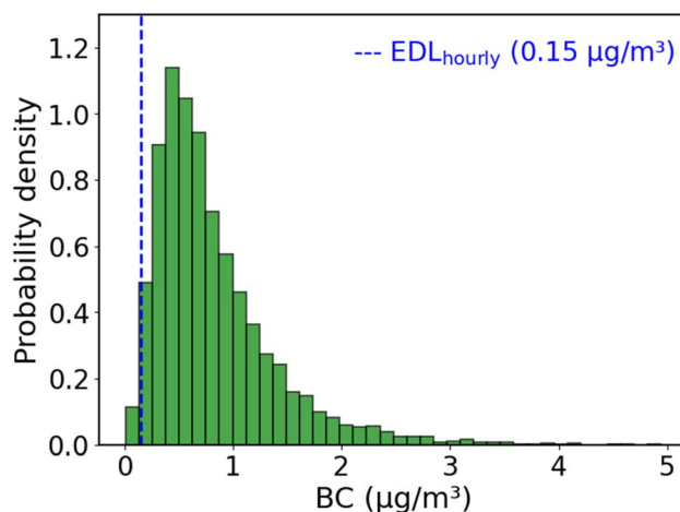
Fig. 4 The histogram plot shows the probability distribution curve of hourly BC for a near-road site (AQ5 ID: 42-003-1376, latitude: 40.437430 and longitude: -79.863572) in Pittsburgh, Pennsylvania (USA). The vertical blue dashed line represents the EDL of the image reflectance method. The monitoring station is a roadside site and BC data is measured with an aethalometer, sampled between August 2020 to July 2021. The hourly BC concentration was higher than the EDL ( 0.15 \mu\text{g m}^{-3} ) more than 98% of the time.
