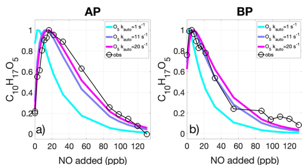
Fig. 4 Normalized traces of the second generation \text{C}_{10}\text{H}_{17}\text{O}_5 peroxy radicals observed during the OH-oxidation of (a) AP and (b) BP, as a function of NO. Conducting numerous simulations to optimize model-observation agreements allowed us to define an optimal range of k_{\text{auto}} for each, which for AP exceeds 20 \text{ s}^{-1} and 11.1 ( 6.2, 16 ) \text{s}^{-1} for BP. Three simulated traces of \text{C}_{10}\text{H}_{17}\text{O}_5 with widely varying rates of their auto-oxidation are shown.
