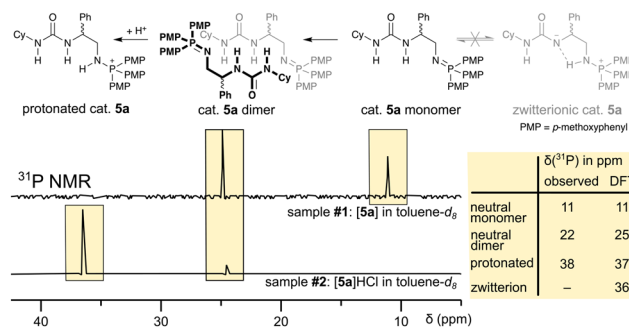
Scheme 2 ^{31}\text{P} NMR spectra of catalyst 5a in toluene- d_8 (top) and with additional HCl (bottom) are assigned to a neutral monomeric, a neutral dimeric, and a protonated species. A zwitterionic species of the catalyst is not observed ( cf. ESI† for sample preparation and DFT calculation).
