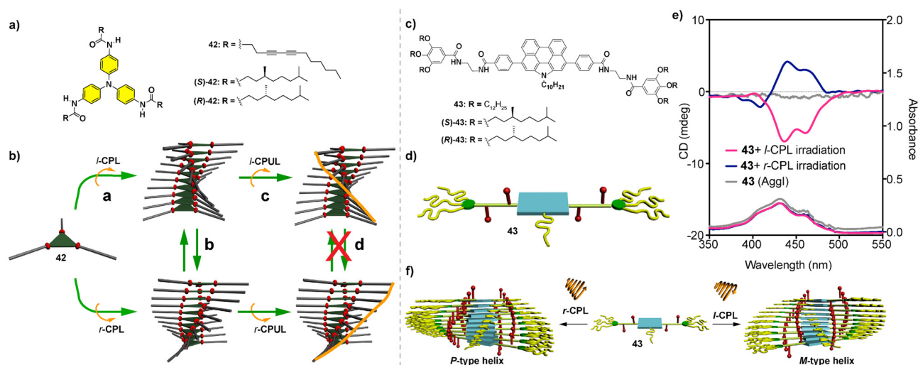
Fig. 22 (a) Chemical structure of triarylamines 42 . (b) Schematic representation of the formation of helical SPs and covalent polymers from 43 upon CPL irradiation. (c) and (d) Chemical structure and schematic illustration of the N-annulated perylenes 43 . (e) UV-Vis (bottom) and CD (top) spectra of the aggregated species formed from 43 upon CPL irradiation. (f) Schematic illustration of the formation of M- or P-type helical SPs upon irradiation of 43 with l -CPL or r -CPL, respectively (reproduced from ref. 110b with permission from the American Chemical Society, copyright 2010).
