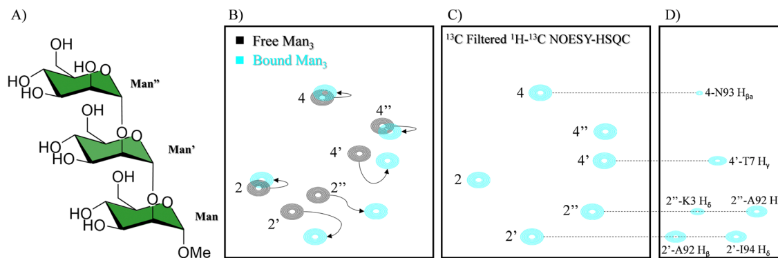
Fig. 22 (A) Scheme of Man 3 . (B) In black 1 H– 13 C HSQC of the 13 C labelled Man 3 and in blue in the presence of CV-N. The shift of the signal is indicated with arrows (C) sugar region of the 13 C filtered NOESY-HSQC (D) side chain region of the 13 C filtered NOESY-HSQC. NOEs between the glycan and CV-N are indicated. Adapted from ref. 131.
