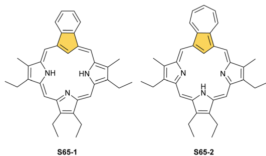
Scheme 65 \beta -Alkylated benzocarporphyrin S65-1 and \beta -alkylated azuliporphyrin S65-2 .
