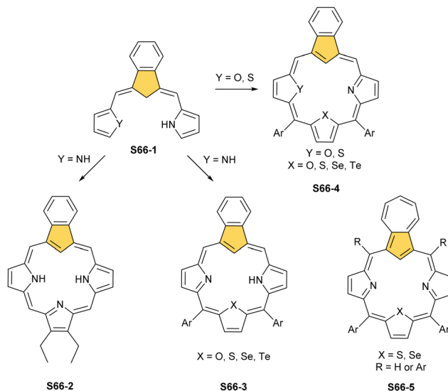
Scheme 66 Synthesis of 23-hetero-, 22,23-dihetero- and regular benzocarporphyrins from carbatripyrrin S66-1 . Respective 23-heteroazuliporphyrin S66-5 .
