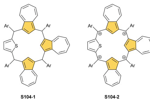
Scheme 104 Triazulporphyrinogens S104-1 and S104-2 .
