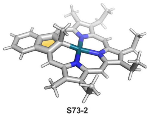
Fig. 17 Palladium(II) C(21)-methylated benzocarporphyrin.
