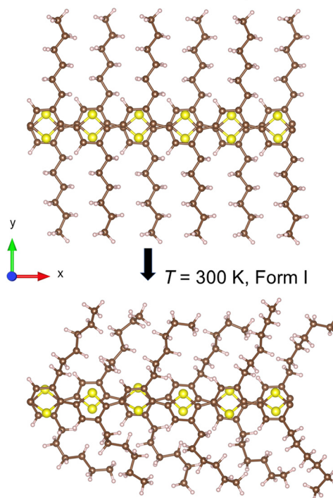
Fig. 12 Evolution of the structure of the periodic system of two P3HT polymers from planar at T = 0 K to Form I at room temperature (representative snapshot, the alkyl chains fluctuating dynamically). View of the system of Fig. 11 on the x - y plane.
