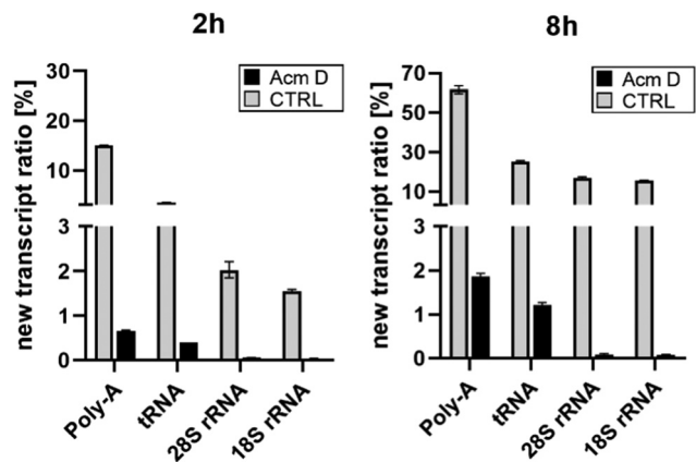
Fig. 2 New transcript ratio (TR) of various RNAs after 2 and 8 hours of 1 \mu\text{M mL}^{-1} AcmD incubation determined by NAIL-MS. Error bars reflect the standard deviation of two biol. replicates.
