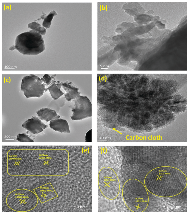
Fig. 4 TEM micrographs of the as-prepared \text{MoO}_2 nanoparticles of (a), (b) N1 and (c), (d) M1 samples; HRTEM micrographs of the (e) N1 and (f) M1 samples.
