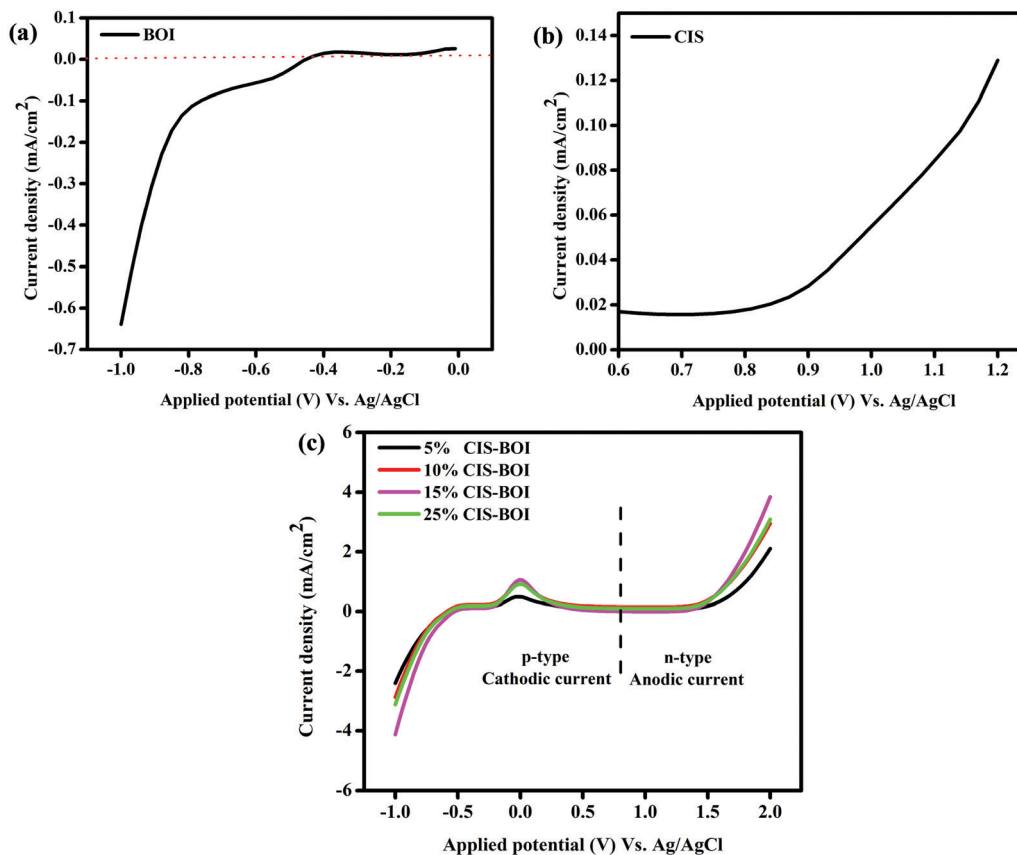
Fig. 9 LSV plots of (a) pristine BOI, (b) pristine CIS, and (c) CIS-BOI composites with varying wt% of CIS.
