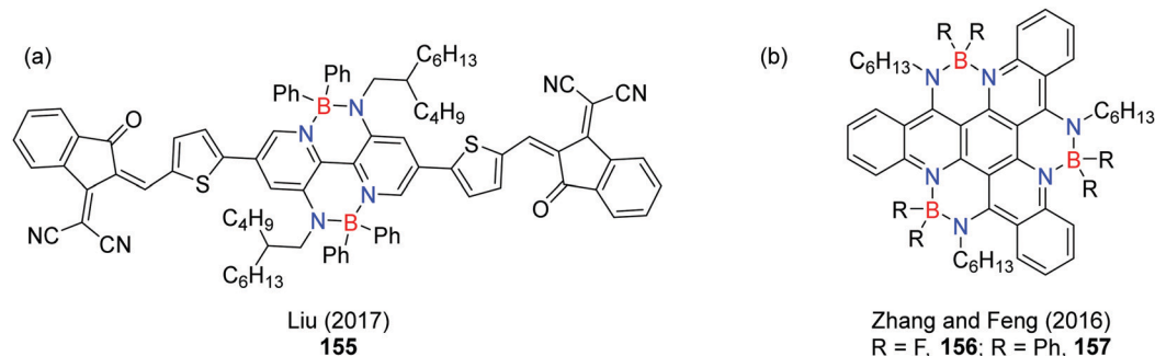
Fig. 48 (a) Doubly NBN-doped pyrene and (b) triply NBN-doped triazatrinaphthylene with tetracoordinate boron atoms.
