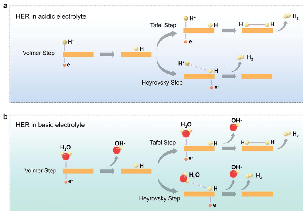
Fig. 3 HER mechanism on a TMDC surface in different electrolytes: (a) acidic solution, (b) alkaline or neutral solution. Hydronium cation ( H_3O^+ ) and a water molecule ( H_2O ) serve as proton donors in the acidic and basic electrolytes, respectively.
