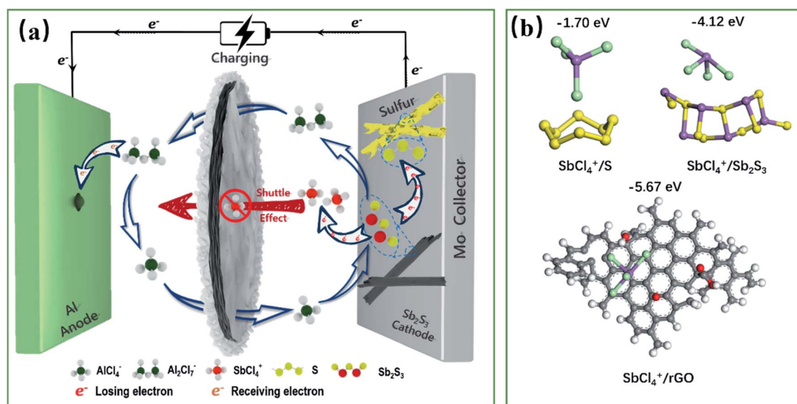
Fig. 4 Schematic diagram of the energy storage mechanism of the Sb 2 S 3 cathode materials during the charging process (a). Theoretical calculations of adsorption energies and structures of SbCl 4 + adsorbed on S, Sb 2 S 3 and rGO (b).
