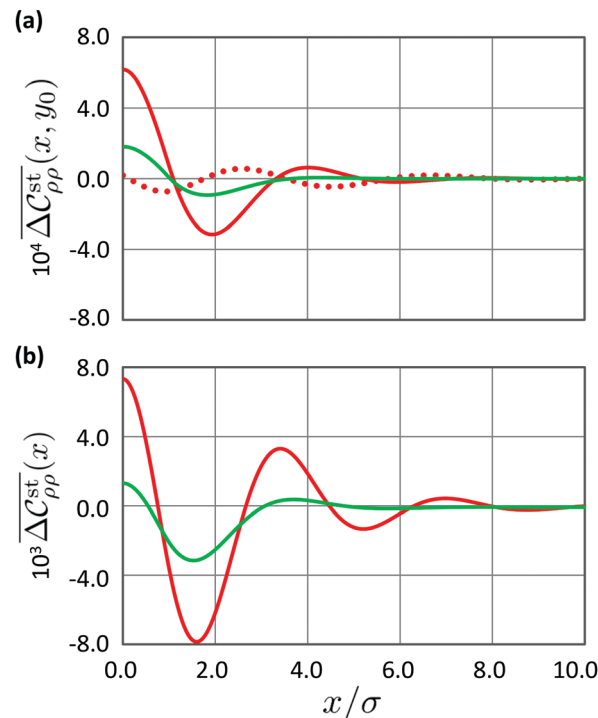
Fig. 5 Comparison between the 1D results of \overline{\Delta C_{\rho\rho}^{\text{st}}}(x, y_0) at a fixed y_0 and \overline{\Delta C_{\rho\rho}^{\text{st}}}(x) defined by eqn (64). The density-density correlation functions are plotted as functions of x/\sigma , the separation distance in the applied field direction measured in units of sphere diameter \sigma . At an identical electric field strength pE\sigma = 0.5 , two ionic concentrations, \bar{\kappa}\sigma = 2.2 and 2.6, are considered in both figures: (a) the green and red solid lines depict the behaviors of \overline{\Delta C_{\rho\rho}^{\text{st}}}(x, y_0 = 0) at \bar{\kappa}\sigma = 2.2 (green) and 2.6 (red), respectively, whereas the red dotted line represents \overline{\Delta C_{\rho\rho}^{\text{st}}}(x, y_0 = 5\sigma) at \bar{\kappa}\sigma = 2.6 ; (b) the green and red solid lines depict the behaviors of \overline{\Delta C_{\rho\rho}^{\text{st}}}(x) at \bar{\kappa}\sigma = 2.2 and 2.6, respectively.
