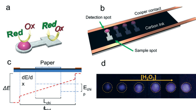
Fig. 1 Schematic representation of the sensor including the principles of SEES. a) Scheme of the paper device indicating the reactions occurring in each spot, b) general overview of the SEES-ECL proposed method, c) diagram showing electrical potential along the electrode, d) real captures of the ECL response using the smartphone. Conditions: 25 V, sample volume: 2.5 \mu L, [H 2 O 2 ] 0.05–150 mM.
