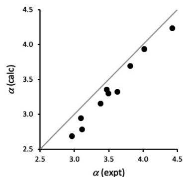
Fig. 9 Comparison of calculated and experimental values of \alpha for compounds 1–10. The line is y = x .
