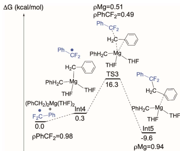
Fig. 7 Computed C–C coupling pathway at MgBn 2 (THF) 2 .
