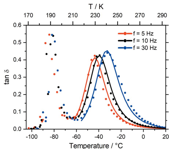
Fig. 7 Loss tangent from the DMTA spectrum of [C_4C_1im][NTf_2] , measured at different frequencies. Solid lines are a concomitant fit, see ESI.†
