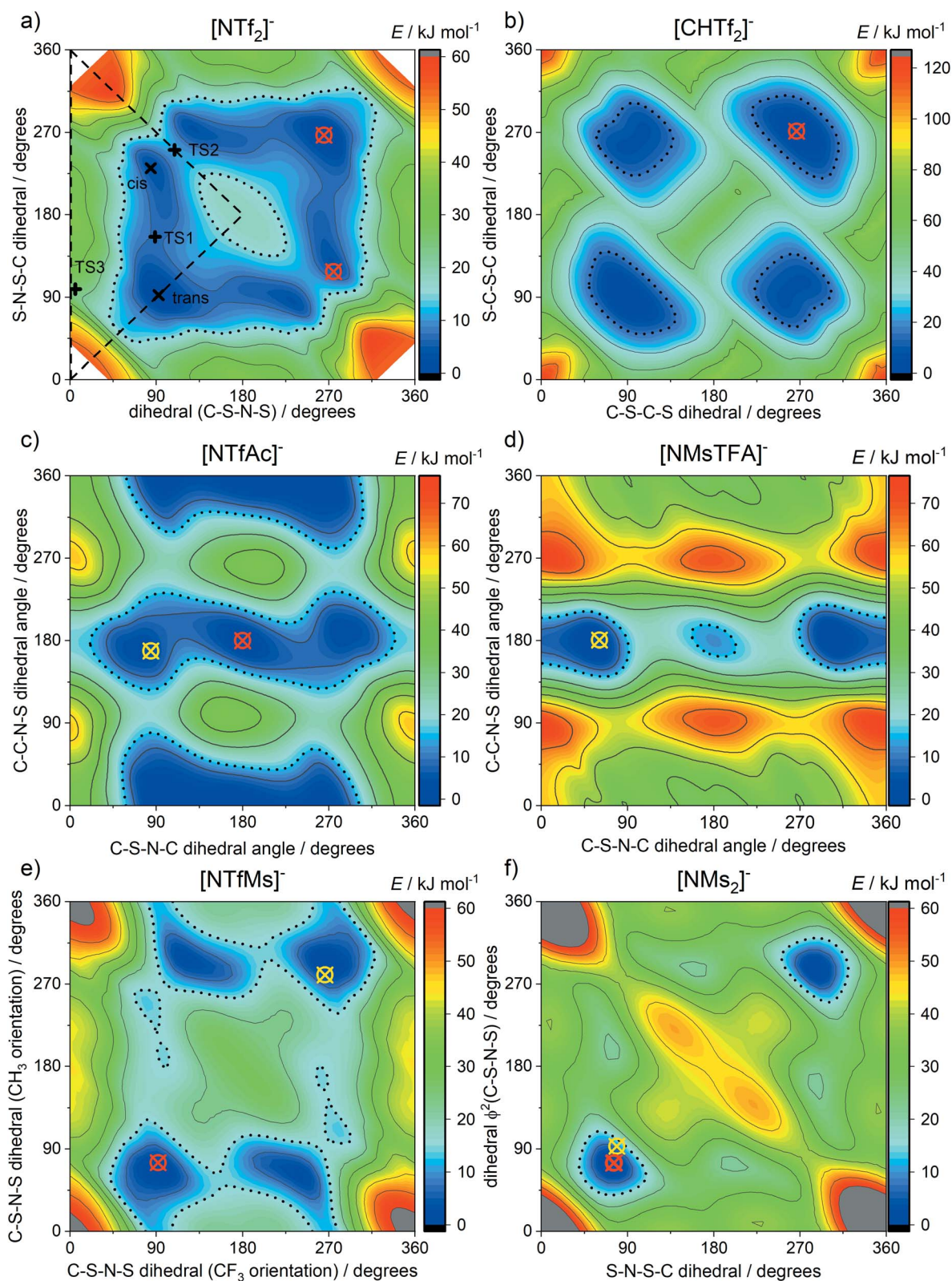
Fig. 3 Potential energy surfaces of (a) [NTf 2 ] − , (b) [CHTf 2 ] − , (c) [NTfAc] − , (d) [NMSTfA] − , (e) [NTfMs] − , (f) [NMs 2 ] − . Crosses indicate experimental dihedral angles obtained from crystal structures, red for anions and yellow for their corresponding free acids. See ESI† for details, and CSD deposition number 236629 and 236630 for [NTf 2 ] − . 101,102 Long dashed lines enclose the symmetrically unique region. The 15 kJ mol −1 isolines are drawn with black dots.
