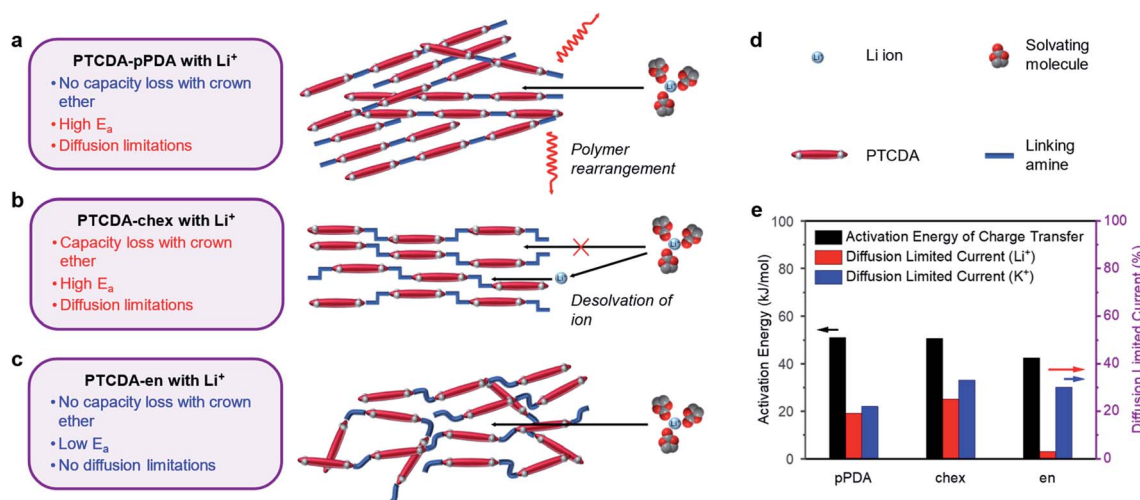
Fig. 6 Schematics for the proposed charge compensation mechanisms for (a) PTCDA-pPDA, (b) PTCDA-chex, and (c) PTCDA-en in \text{Li}^+ containing electrolyte solutions. The black arrows represent ion diffusion, and the red arrows represent polymer diffusion/rearrangement. (d) Legend corresponding to a–c. (e) Bar chart summarizing the activation energy of charge transfer with \text{Li}^+ and diffusion-limited current proportion in \text{Li}^+ and \text{K}^+ batteries based on CV tests for the PDI-based polymers.
