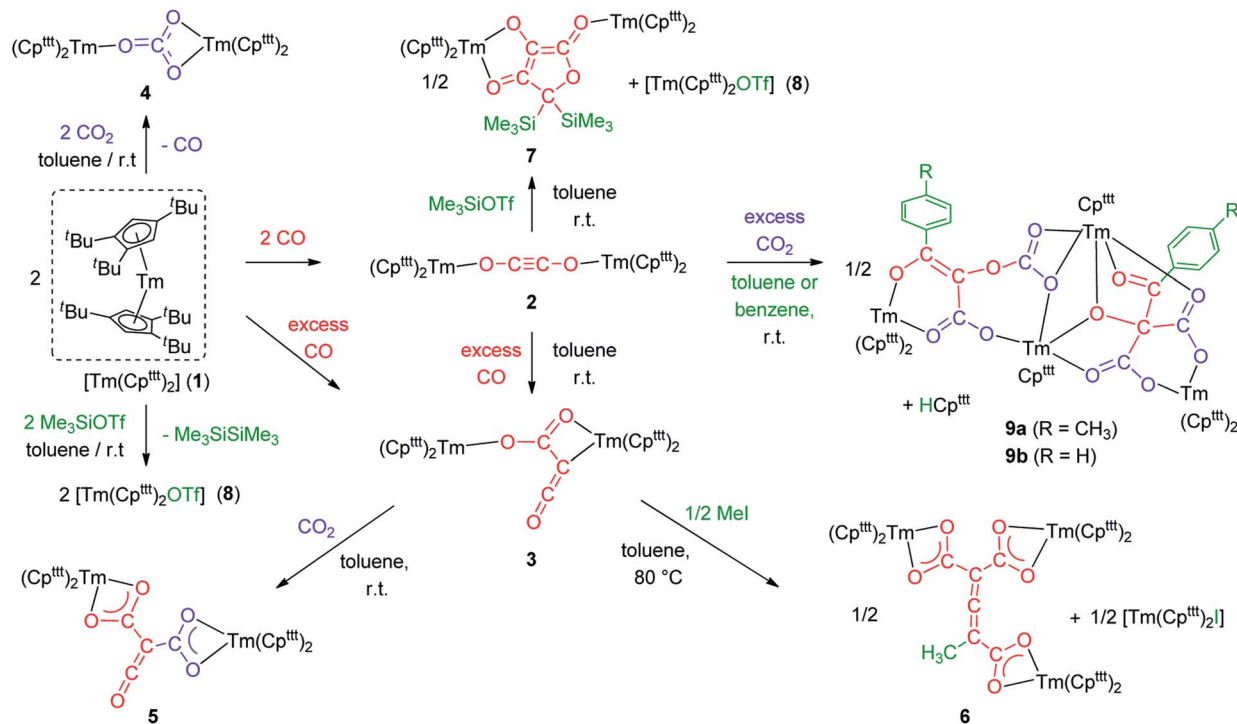
Scheme 5 Summary scheme of all the reactivity described in this study starting from [Tm(Cp^{ttt})_2]_2 (1).
