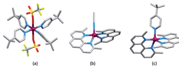
Fig. 4 The structures of (a) trans -[Cu(TBP) 4 (O 3 SCF 3 ) 2 ] (CSD 120 refcode IPEWAD), (b) the [Cu(Me 2 phen) 2 (NCMe)] 2+ cation in the perchlorate salt (CSD refcode XIDWEP), and (c) the [Cu(Me 2 phen) 2 (TBP)] 2+ cation from the structure of the TFSI - salt; the cif was kindly provided by the authors of ref. 119. Hydrogen atoms are omitted for clarity. As a general note, 3D-structures in this review have been drawn using coordinates retrieved from the Cambridge Structural Database (CSD, version 2021.2.0) 121 and using Mercury version 2021.2.0. 122
