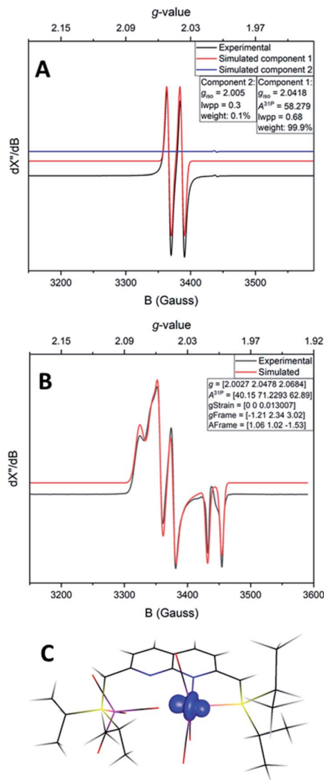
Fig. 4 Experimental (black) and simulated (red) X-band EPR spectrum of 7 in toluene at room temperature (A) or in a toluene glass at 30 K (B). (A) Microwave freq. 9.649849 GHz, mod. amp. 4.000 G, power 0.6325 mW. Simulation parameters component 1 (7): g_{\text{iso}} = 2.0418 , A^{31\text{P}} = 58.279 MHz, Gaussian line broadening 0.68 mT, weight = 99.9%. Simulation parameters component 2 (TBP): g_{\text{iso}} = 2.005 , Gaussian line broadening 0.3 mT, weight = 0.1%. (B) Microwave freq. 9.650852 GHz, mod. amp. 2.000 G, power 0.2000 mW. Simulation parameters: g [2.0027, 2.0478, 2.0684], A^{31\text{P}} [40.15, 71.2293, 62.89], g -strain [0, 0, 0.013007], g -frame [-1.21, 2.34, 3.02], A -frame [1.06, 1.02, -1.53]. (C) The structure of 7 and its spin density plot (isosurface value of 0.02 e Bohr -3 ).
