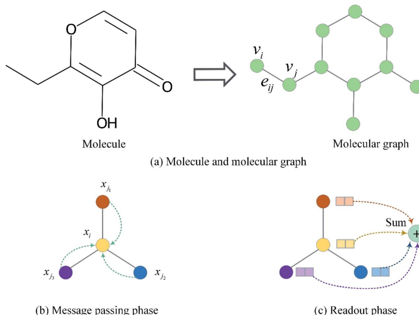
Fig. 3 Molecule representation and graph embedding. (a) Representing a molecule as a graph. (b) Graph message passing phase corresponding eqn (1). (c) Graph readout phase corresponding eqn (2).
