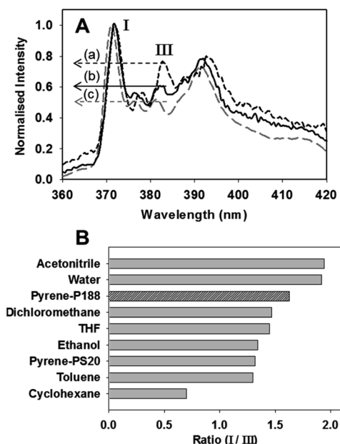
Fig. 12 Determination of microenvironment polarity within \text{P}_{188} nanoparticles using pyrene as ratiometric emission probe. (A) Fluorescence spectra at rt of (a) pyrene in toluene (b) aqueous pyrene- \text{P}_{188} (NP-pyrene- \text{P}_{188} ) (c) pyrene in water, with the first (I) and third (III) identified. (B) Ratiometric values for pyrene emission first (I) and third (III) bands in organic solvents of varying polarity and water, aqueous \text{P}_{188} and aqueous \text{PS}_{20} .
