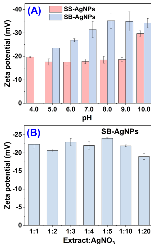
Fig. 4 The \zeta -potential of AgNPs obtained at different (A) pH; (B) material ratios.
