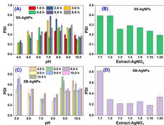
Fig. 3 Polydispersity index (PDI) of SS-AgNPs and SB-AgNPs obtained with different process parameters. (A) and (C) have different pH and incubation times; (B) and (D) have different material ratios.
