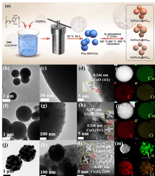
Fig. 1 (a) Schematic illustration of the preparation of polyMOF(Co) and the series of \text{Co/Co}_x\text{O}_y\text{@mC} by calcining polyMOF(Co) at different temperature of 400 °C, 600 °C, and 800 °C under \text{N}_2 atmosphere. TEM images and HAADF image, element mappings (Co (green), C (red), and O (orange)) of (b–e) \text{Co/Co}_x\text{O}_y\text{@mC}_{400} , (f–i) \text{Co/Co}_x\text{O}_y\text{@mC}_{600} , and (j–m) \text{Co/Co}_x\text{O}_y\text{@mC}_{800} hybrids.
