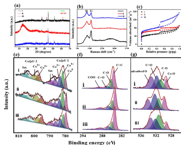
Fig. 2 (a) XRD patterns, (b) Raman spectra, (c) \text{N}_2 adsorption-desorption isotherms, and the high-resolution (e) Co 2p, (f) C 1s and (g) O 1s XPS spectra of (i) \text{Co/Co}_x\text{O}_y\text{@mC}_{400} , (ii) \text{Co/Co}_x\text{O}_y\text{@mC}_{600} , and (iii) \text{Co/Co}_x\text{O}_y\text{@mC}_{800} .
