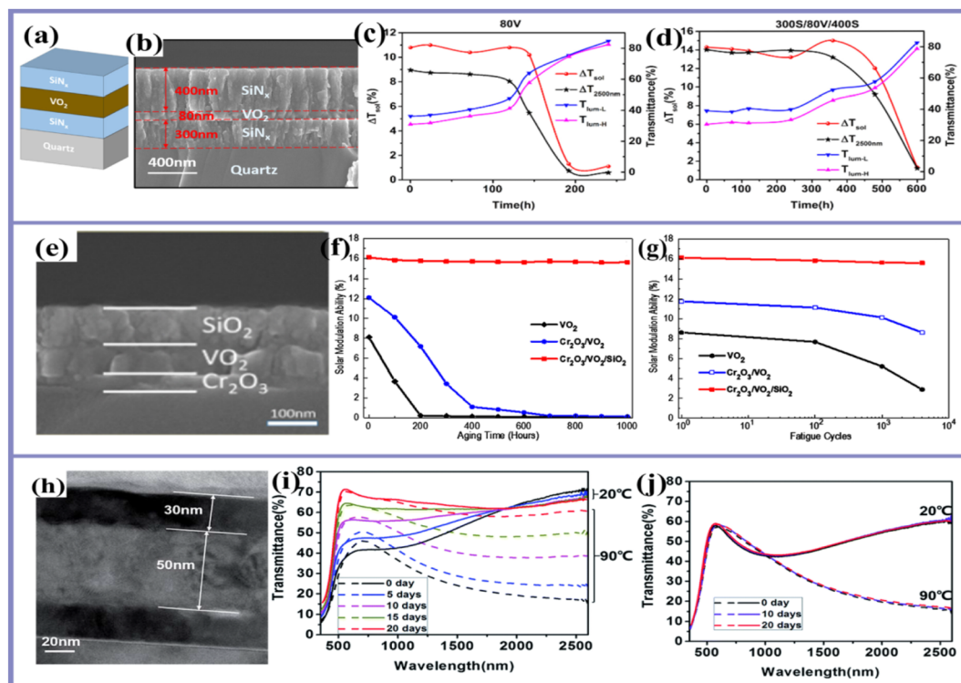
Fig. 8 (a) Preparation of SiN x /VO 2 (SV), VO 2 /SiN x (VS), and SiN x /VO 2 /SiN x (SVS) multilayers by using the reactive magnetron sputtering method. (b) Field Emission Scanning Electron Microscopy (FE-SEM) of the multilayers. (c) Durability graph of the SVS film at 60 °C and humidity of 90%. (d) Comparison graph of the aging test. Reproduced with permission 136 Copyright © 2018, Elsevier. (e) Preparation of the sandwiched structure of Cr 2 O 3 /VO 2 /SiO 2 (CVS) on a glass substrate by using the magnetron sputtering process and SEM images. (f) Fatigue test of simple VO 2 and structures. (g) Comparison graph of single VO 2 layer and SVS layers. Reproduced with permission 137 Copyright © 2017, Elsevier. (h) SEM image of the as prepared sandwiched structure of VO 3 /VO 2 /WO 3 on VO 2 by using the medium frequency reactive magnetron sputtering technique (MFRMST) and HRTEM images. (i) Durability graph of the prepared layer under different temperature and humidity conditions. (j) Aging test of the VO 2 sample and thin-film WO 3 /VO 2 /WO 3 . Reproduced with permission 138 Copyright © 2016, The Royal Society of Chemistry.
