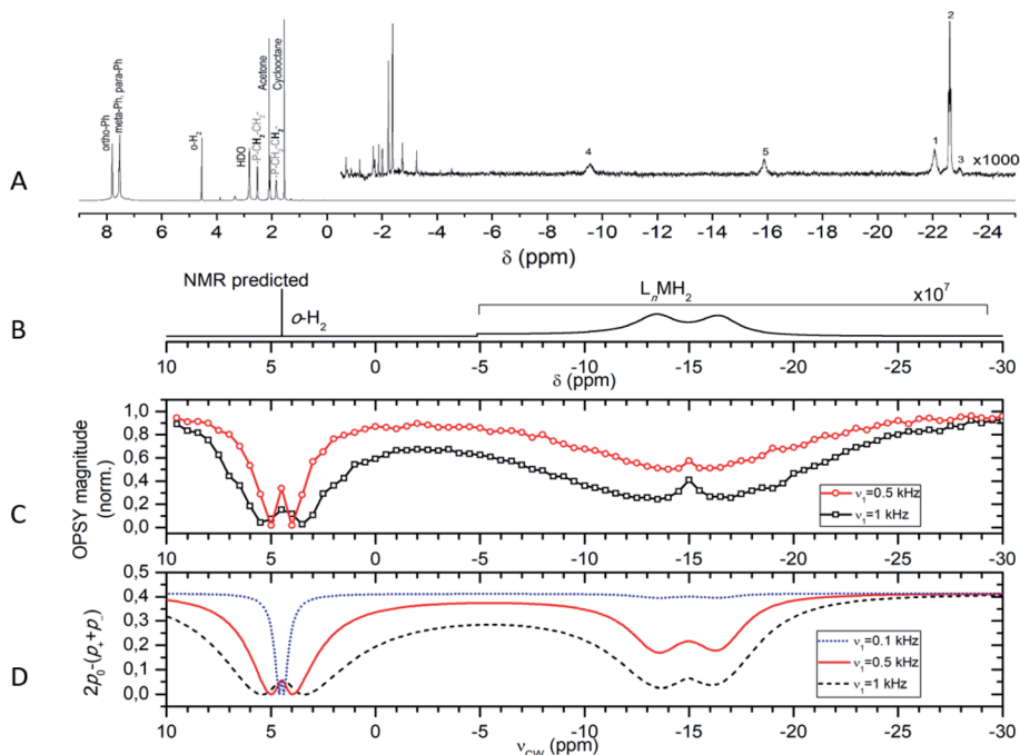
Fig. 11 (A) Thermal 700 MHz 1 H NMR spectrum accumulated after bubbling the catalyst solution by n\text{-H}_2 (512 scans, 30 minutes) and magnification ( \times 1000 ) of the dihydrogen and dihydride region. Note that there is no signal of any complex between catalyst and hydrogen. (C and D) Experimental and simulated PANEL spectra, showing the signal of the hidden complex (lines at -16.5 ppm and -13.5 ppm). (B) Calculated NMR spectrum of the hidden complex, magnified by factor 10^7 (for details see Kiryutin et al. 93 ).
