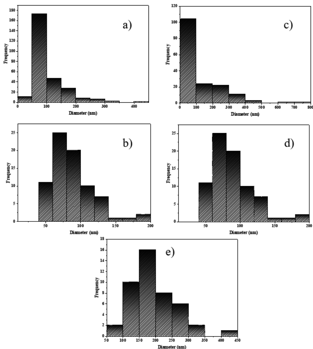
Fig. 3 The particle size distribution histogram of \text{NaY}(\text{WO}_4)_2 samples prepared by (a) glucose, (b) fructose, (c) lactose, (d) cellulose, and (e) starch using Digimizer as the image analyser.
