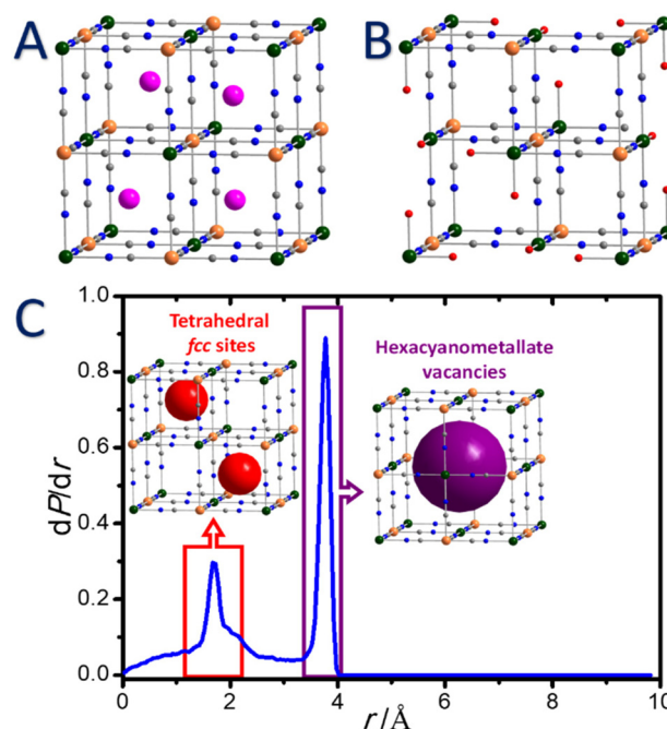
Fig. 1 Crystalline structure of non-lacunar (A) and lacunar (B) PBA, A_{1-x}M[M'(CN)_6]_{1-x/3}nH_2O . Colour code: orange, M' ; green, M ; magenta, A^I ; blue, N ; grey, C . The oxygen of H_2O coordinated to the M'^{2+} ions are represented by red spheres; (C) pore size distribution of PBA obtained from Monte Carlo simulations illustrating the presence of two types of pores corresponding to the tetrahedral sites of the fcc structure and the larger pores formed by hexacyanometallate vacancies.
