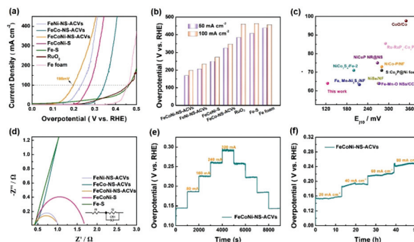
Fig. 3 Electrochemical measurements: (a) OER polarization curves, (b) overpotential comparison at 50\text{ mA cm}^{-2} and 100\text{ mA cm}^{-2} , (c) comparison of the overpotentials ( E_{10} ) and Tafel slopes with the references, (d) Nyquist plots, and (e and f) stability tests of the obtained catalysts in 1 M KOH.
