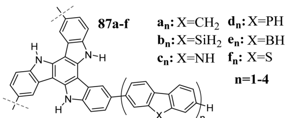
Scheme 30 Tri(oligoheterofluorene) 5,10,15-triazatruxenes.
