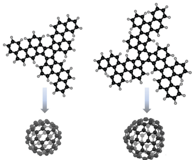
Fig. 3 Truxene-based fullerenes precursors: left – \text{C}_{60} and right – \text{C}_{84} .
