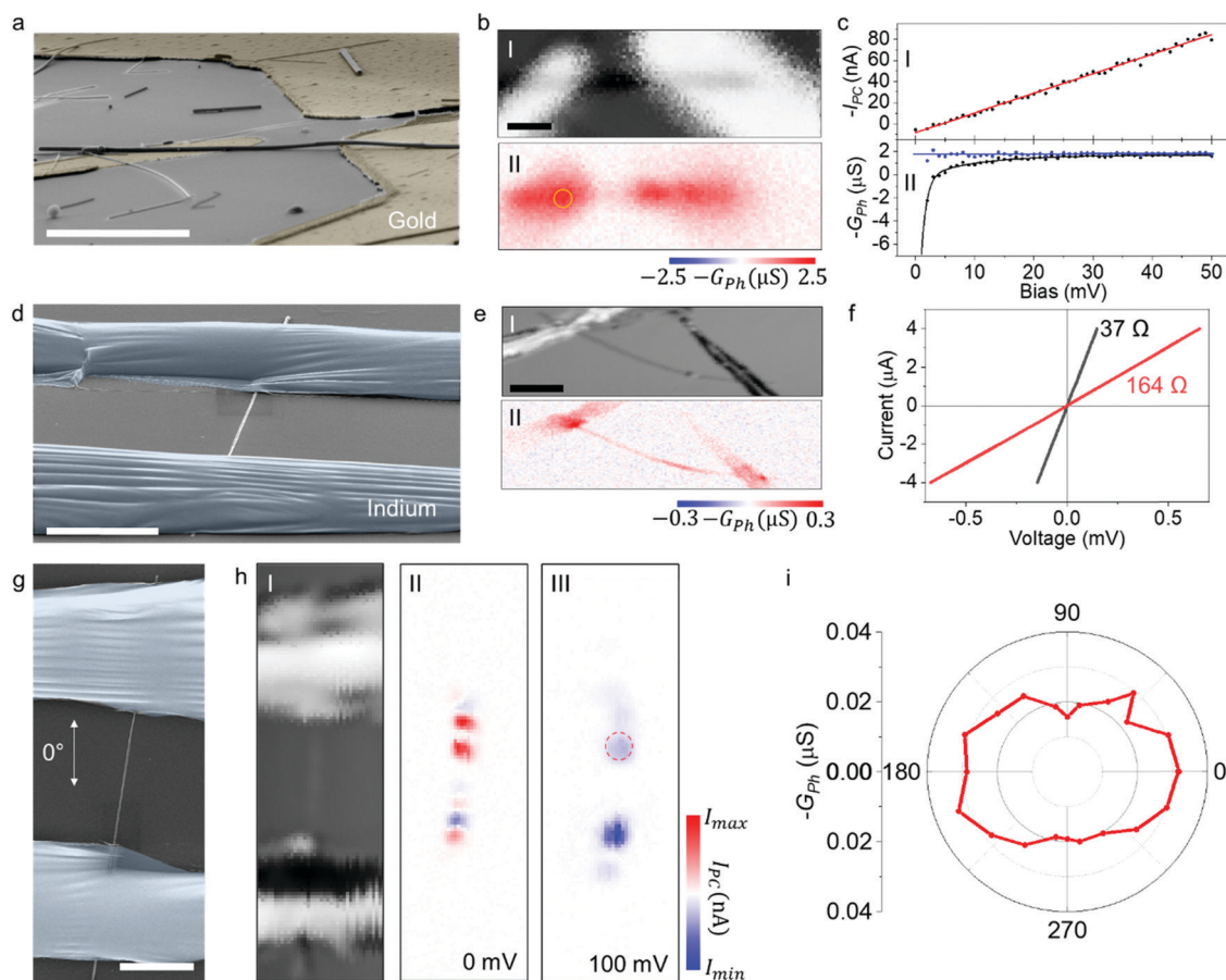
Fig. 3 (a) False colored SEM image of a Ag NW on pre-patterned gold electrodes. Scale bar is 5 \mu\text{m} . (b) Reflection map (I) and the corresponding -G_{\text{ph}} map under 20 mV bias (II) showing the photoconductance over the device. It is noteworthy that there is a significant conductance modulation over the gold electrodes. A 532 nm laser source was used at 65 \mu\text{W} power. The yellow circle indicates the position where -I_{\text{PC}} vs. bias measurements were taken from. The scale bar is 5 \mu\text{m} . (c) -I_{\text{PC}} vs. bias (I) graph showing a linearly increasing -I_{\text{PC}} with the bias (black dots). The red line is the linear fit to the data. Zero bias response is \sim 6 nA. Lower panel (II) shows -G_{\text{ph}} (black dots) and -\frac{I_{\text{PC}} - I_{\text{PC}}^0}{V} (blue dots) vs. bias. Solid lines are fits to the data. (d) False colored SEM image of an indium contacted Ag NW. Note the grating-like structures over the indium, which naturally occur due to thermal contraction upon cooling. Scale bar is 5 \mu\text{m} . (e) Reflection map (I) and the corresponding -G_{\text{ph}} map under 100 mV bias (II) showing the conductance modulation over the indium contacts. Notice that the modulation intensifies near the indium-NW junction. Also, the visible defect in the reflection map results in enhanced plasmonic response, which is clear in the photoconductance map. Data were collected with a 532 nm laser at 96 \mu\text{W} . Scale bar is 10 \mu\text{m} . (f) Current vs. voltage graphs of the same devices, before (red dots) and after (black dots) reduction of the photoconductance. (g) False colored SEM image of a device with the incident polarization angle marked. (h) (I) Reflection map, (II) open-circuit response, and (III) 100 mV response maps are shown. I_{\text{max}} = 0.25 nA for (II), 25 nA for (III) and I_{\text{min}} = -0.25 nA for (II) and -25 nA for (III). (i) The polar chart shows the incident polarization angle vs. -G_{\text{ph}} at 100 mV bias. The data were collected from the individual maps taken around the red dashed circle in h (III).
