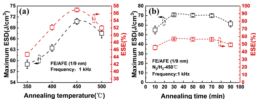
Fig. 3 The maximum ESD and corresponding ESE of the capacitor with the FE (1 nm)/AFE (9 nm) stack: (a) at different annealing temperatures for 30 \text{ min} ; (b) at 450 \text{ } ^\circ\text{C} for different annealing times. Ten devices are measured for each sample.
