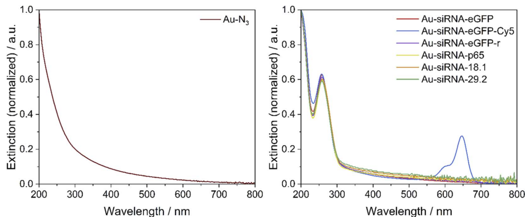
Fig. 3 UV-Vis spectra of azide-terminated gold nanoparticles ( \text{Au-N}_3 , left) and of siRNA-functionalized gold nanoparticles (right). The absorption of RNA is visible by the band at 258 nm. The absorption of Cy5 is visible by the band at 647 nm.
