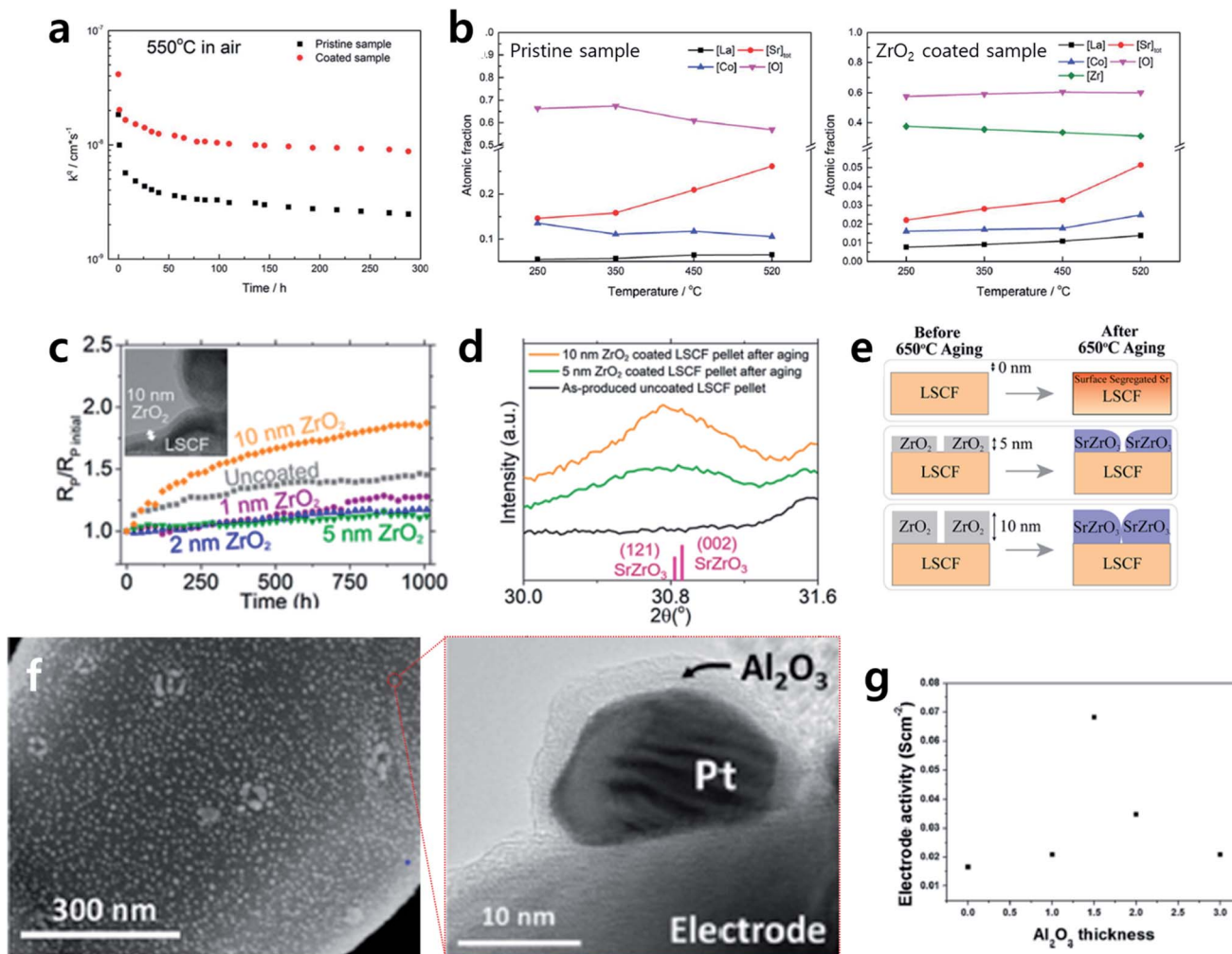
Fig. 7 (a) Time evolution of surface oxygen exchange coefficient of \text{La}_{0.6}\text{Sr}_{0.4}\text{Co}_{0.8}\text{Fe}_{0.2}\text{O}_{3-x} film electrode with and without \text{ZrO}_2 ALD coating. (b) Temperature dependent atomic concentrations of pristine and \text{ZrO}_2 coated \text{La}_{0.6}\text{Sr}_{0.4}\text{Co}_{0.8}\text{Fe}_{0.2}\text{O}_{3-x} electrode. (c) Aging behavior of normalized polarization resistance depending on the thickness of \text{ZrO}_2 ALD coating. (d) X-ray diffraction patterns obtained from pristine \text{La}_{0.6}\text{Sr}_{0.4}\text{Co}_{0.8}\text{Fe}_{0.2}\text{O}_{3-x} , 5 nm \text{ZrO}_2 coated \text{La}_{0.6}\text{Sr}_{0.4}\text{Co}_{0.8}\text{Fe}_{0.2}\text{O}_{3-x} , and 10 nm \text{ZrO}_2 coated \text{La}_{0.6}\text{Sr}_{0.4}\text{Co}_{0.8}\text{Fe}_{0.2}\text{O}_{3-x} pellets after aging. (e) Schematics of proposed degradation mechanisms for uncoated and \text{ZrO}_2 coated \text{La}_{0.6}\text{Sr}_{0.4}\text{Co}_{0.8}\text{Fe}_{0.2}\text{O}_{3-x} . (f) SEM image of Pt nanocatalysts decorated \text{La}_{0.75}\text{Sr}_{0.25}\text{Cr}_{0.5}\text{Mn}_{0.5}\text{O}_{3-x} electrode and TEM image of encapsulated Pt nanocatalysts by \text{Al}_2\text{O}_3 . (g) Electrode activity for \text{CH}_4 fuel oxidation of \text{La}_{0.75}\text{Sr}_{0.25}\text{Cr}_{0.5}\text{Mn}_{0.5}\text{O}_{3-x} according to the thickness of \text{Al}_2\text{O}_3 coating. Figures reproduced with permission from ref. 30, 61, and 62. Copyright 2018, The Royal Society of Chemistry, and Copyright 2020, American Chemical Society.
