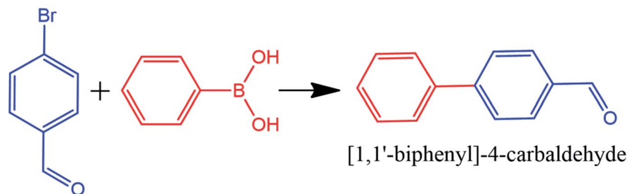
Fig. 4 Suzuki cross-coupling reaction with Pd- \text{Fe}_3\text{O}_4 /RGO heterogeneous catalyst. This figure was adapted with permission from H. A. Elazab, 2019 (DOI: 10.9767/bcrec.14.3.3518.478-489). 50
