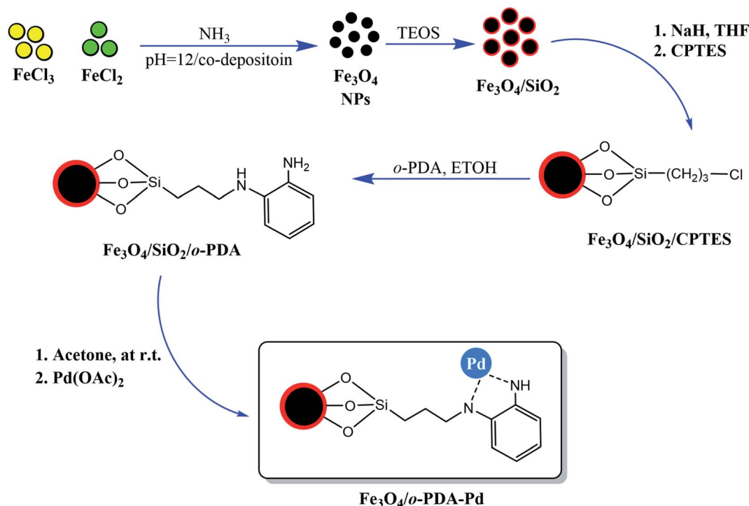
Fig. 5 Preparation of \text{Fe}_3\text{O}_4 /o-PDA-Pd heterogeneous magnetic nanocatalyst. This figure was adapted with permission from Journal of Physics and Chemistry of Solids , 2020, 136 , 109200. 17
