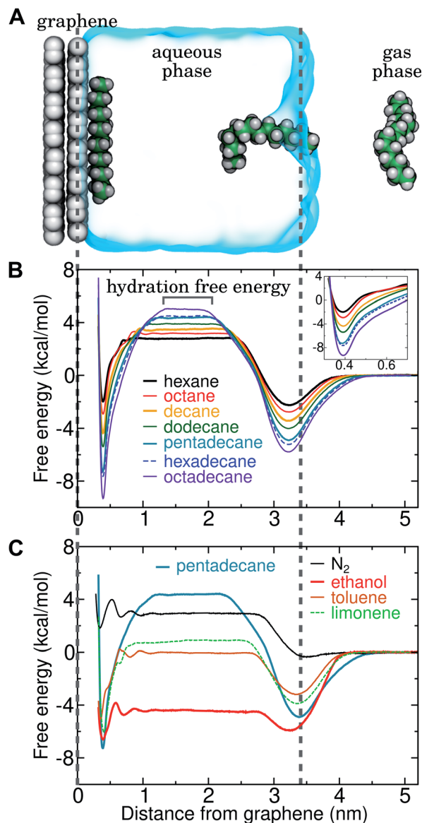
Fig. 4 Simultaneous calculation of the free energy for hydration and adsorption at the graphene–water interface for N 2 and several VOCs. (A) Example simulation system including graphene, water, a gas phase region, and a single molecule of pentadecane. Snapshots of the pentadecane molecule at three different times are shown. (B) Potentials of mean force as a function of distance from the graphene–water interface for a set of straight-chain alkanes. The value of this potential of mean force at a distance of 1.5 nm indicates the calculated hydration free energy for the given molecule. (Inset) Magnified view of the free energy minima at the graphene surface. (C) Potentials of mean force as a function of distance from the graphene–water interface for some common VOCs and N 2 (using the Peng–SPCE model).
