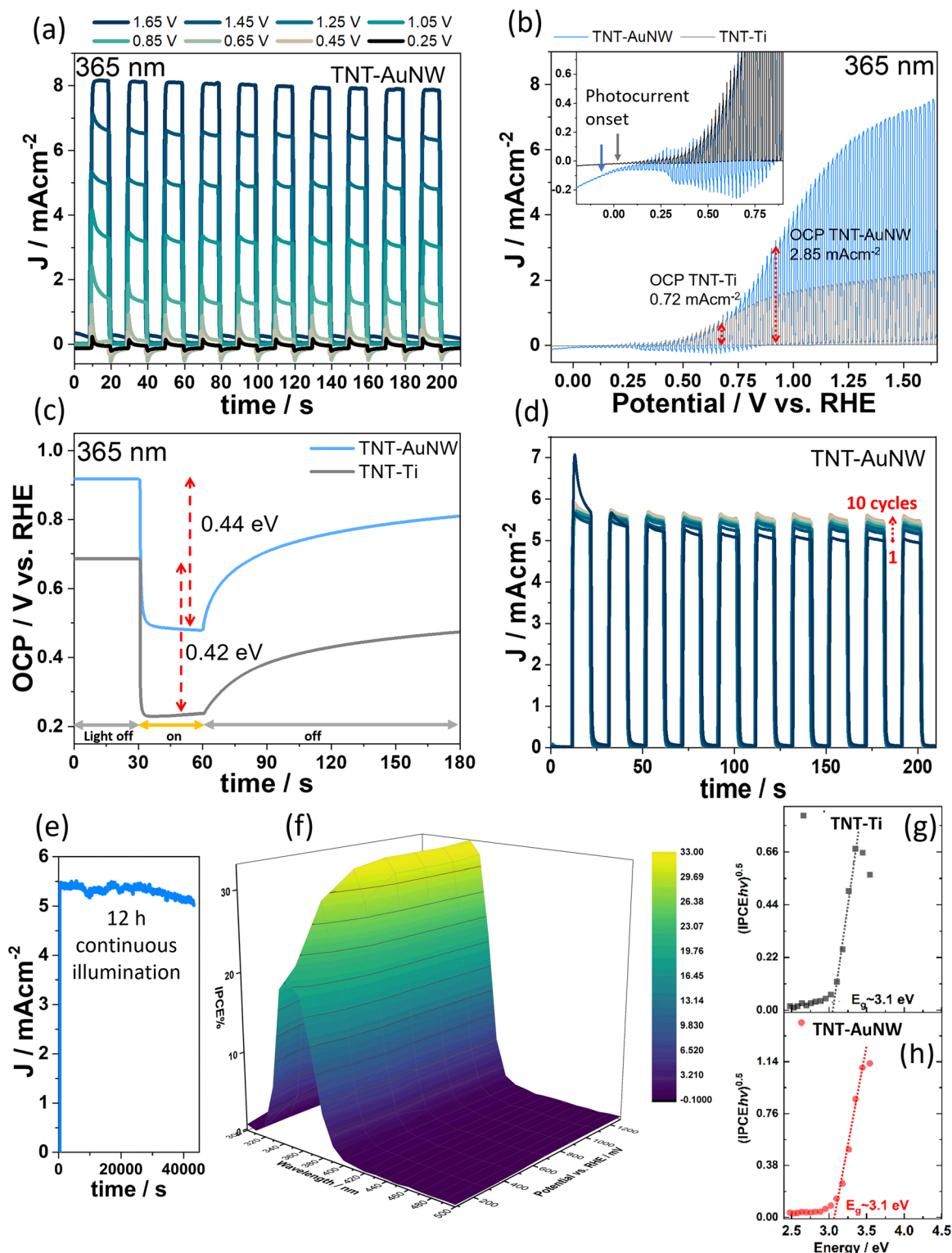
Fig. 4 (a) Transient photocurrent responses of the TNT-AuNW photoanode measured under 365 nm LED illumination and varied constant potentials in the range from 0.25 to 1.65 V vs. RHE in a 0.1 M Na 2 SO 4 solution. (b) Linear sweep voltammograms registered under chopped light illumination (365 nm) from TNT-AuNW and TNT-Ti reference samples. (c) Open circuit potential (OCP) of the photoanodes measured under dark and UV illumination. Stability test of the TNT-AuNW electrode under (d) chopped light and (e) continuous 12 h illumination with 365 nm. (f) IPCE 3D photoactivity map measured for TNT-AuNW. Evaluated band gaps of (g) TNT on Ti and (h) TNT on AuNW from IPCE data given in Fig. S5 (ESI†).
