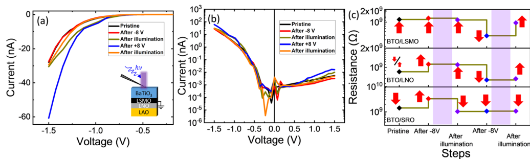
Fig. 6 (a) I-V characteristic of the BTO/LSMO sample in the pristine state and after \pm 8 V prepoling and after \pm 8 V prepoling and subsequent illumination. (b) The same I-V characteristics with current in semi-log scale. (c) Resistance state measured at -1.5 V for the BTO/LSMO, BTO/LNO and BTO/SRO samples after application of \pm 8 V prepoling or illumination as indicated.
