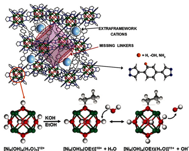
Fig. 7 Top: Schematic representation of the structure of the \text{K}[\text{Ni}_8(\text{OH})_5(\text{EtO})(\text{BDP-X})_{5.5}] systems. Bottom: Cluster deprotonation taking place during the conversion into \text{K}[\text{Ni}_8(\text{OH})_5(\text{EtO})(\text{BDP-X})_{5.5}] materials and proposed proton transfer mechanism to explain the ion conductivity of the hydrated materials. Figure reproduced with permission from [111].
