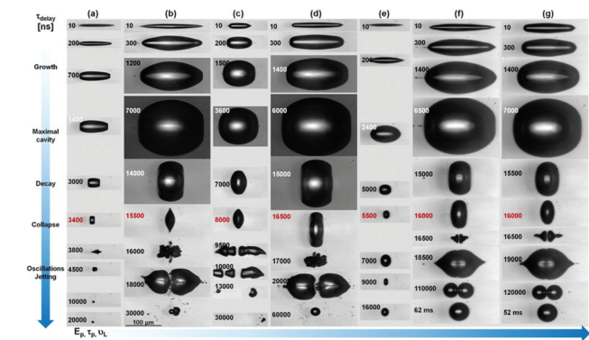
Fig. 14 Two-color pump–probe time-resolved microscopy technique using a random laser as probe laser. A kaleidoscope of cavitation collapse phenomena resulting in directional jetting, bubble stabilization, or fragmentation can be obtained. (Reproduced from ref. 15, with permission from [Springer Nature]).
